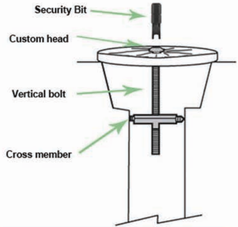
Lock and Stop Diagram (side view of drain)
